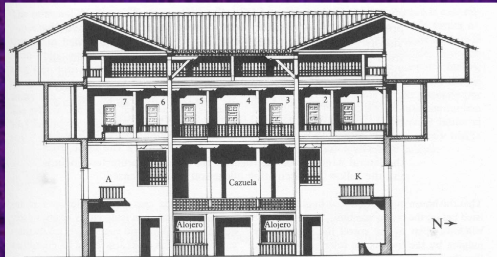
26. Section drawing of the facade boxes in Dorremocha. [J. J. Allen and Carlos
